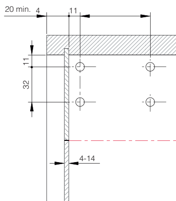
DRILLING PLAN WITHOUT BACK PANEL
